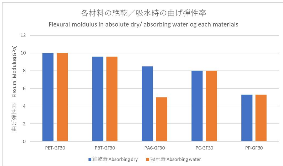
Dry/Conditioned Flexural Modulus for Various Materials
