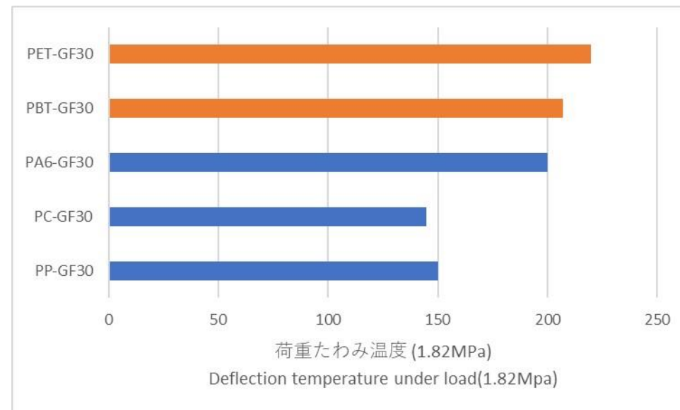
Heat Deflection Temperature of Various Materials
