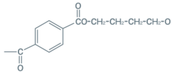
Structural formula of PBT
